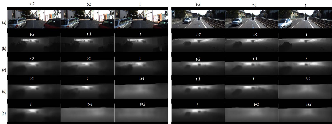
Figure 5: Qualitative demonstration of depth prediction results for the current image frame and future image frames obtained by unfolding the LSTM layers (a) Images at times t_{n-2}, t_{n-1}, t_n , (b) The corresponding ground truth depth maps (c) Depth predictions of the proposed ConvLSTM network for image frames at time steps t_{n-2}, t_{n-1}, t_n (which is the way the network is actually trained to predict) (d) Predictions of the proposed ConvLSTM network, for future frames at time t_{n-1}, t_n, t_{n+1} (e) predictions of the proposed ConvLSTM network for future frames at time t_n, t_{n+1}, t_{n+2} . For (d) & (e), it must be noted that, the proposed ConvLSTM network is not trained to predict future frames; instead we mask the inputs for specific time steps and force the network to predict the frames, thereby exploiting its recurrent nature. Qualitative analysis of the results over several images showed that the proposed network was able to reliably estimate the layout of the scene, but failed to interpolate accurately the motion of the scene objects into the future.
